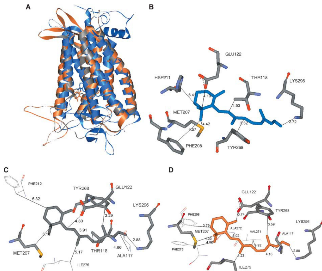
FIGURE 9 (A–D) Comparison of predicted binding sites for retinal (those residues within 5 Å of retinal that interact strongly with the ligand (contributions to binding >1 kcal/mol) before Schiff base bond formation in the three rhodopsin structures. (A) All three structures and ligand conformations are shown. The colors blue, gray, and orange correspond respectively to those structures analyzed in B–D. (B) NoSB-Ret(HD)/closed(xtal) structure. Here we see that seven residues bind more strongly than 1 kcal/mol. (C) NoSB-Ret(HD)/closed(MS). Here we see that five of the seven residues in B are predicted (only Phe-208 and Hsp-211, both rather weakly bound). We also find three additional residues (Phe-212, Ile-275, and Ala-117) that do not bind with 1 kcal/mol in B. (D) NoSB-Ret(HD)/open(MS). Here we see that six of the seven residues in C bind more strongly than 1 kcal/mol. We also find four additional residues that do not bind with 1 kcal/mol in B. This difference results from the shift in the retinal binding site upon closure of the EC-II loop. The side chains in common with the NoSB-Ret(HD)/closed(xtal) structure (in B) or with NoSB-Ret(HD)/closed(MS) (in C) within the binding site around the 11- cis -retinal are labeled with larger type.
