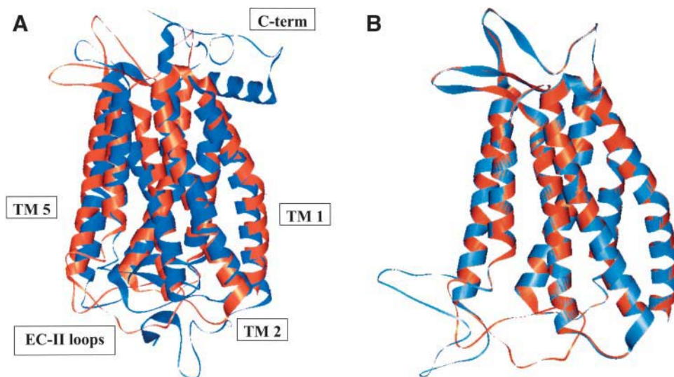
FIGURE 7 (A) Comparison of the predicted structure (orange) Apo/closed(MS) with the experimental structure (blue) Apo/closed(xray). They differ in the TM helical region by CRMS = 2.84 Å. (B) Comparison of the predicted Apo/closed(MS) structure (orange) with the predicted Apo/open(MS) structure (blue). They differ in the TM helical region by 0.11 Å.
